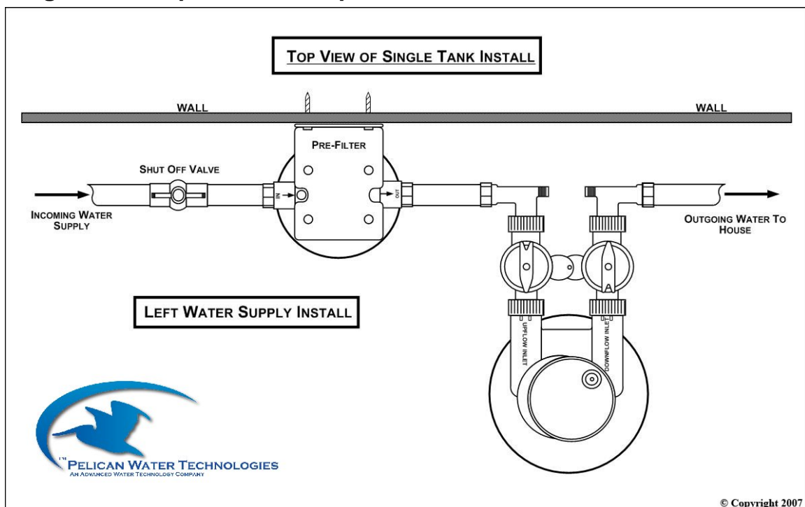
Diagram 7 – Top view of completed installation
